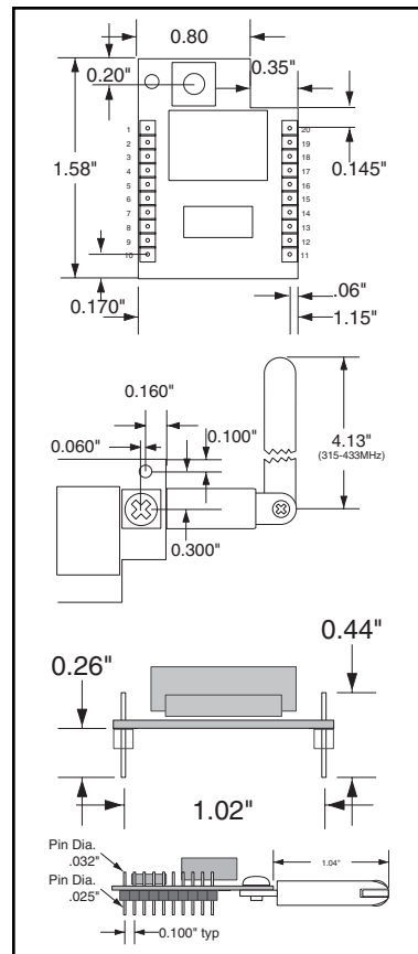
Figure 1: Physical Dimensions
