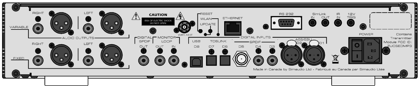
Figure 2: Nëo 380D Rear panel
