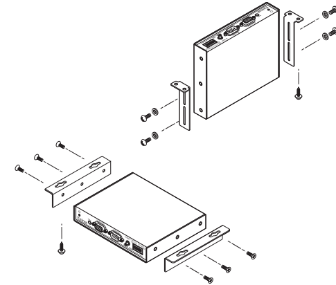
Figure 2-1 — Under-desk mounting
