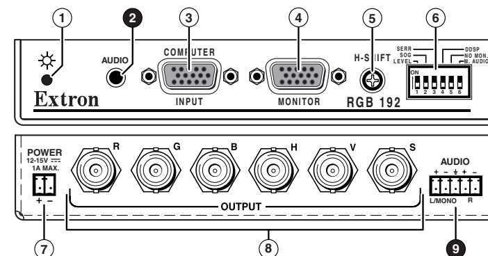
Figure 2-4 — RGB 192 front and rear panel features
