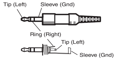
Figure 2-6 — Audio input connector wiring
