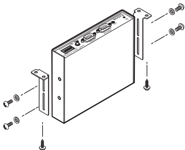
Figure 2-2 — Through-desk mounting
