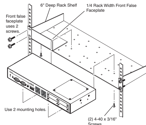
Figure 2-3 — Rack mounting
