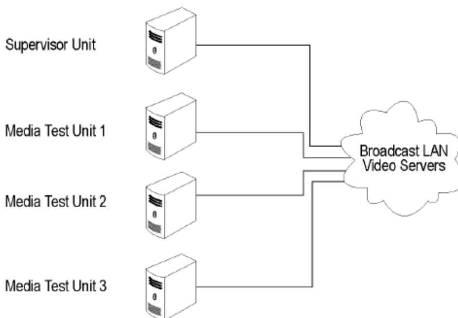
Clustering topology
