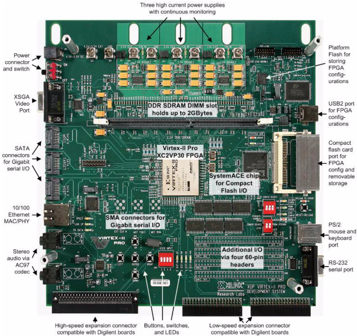
Figure 1-2: XUP Virtex-II Pro Development System Board Photo
