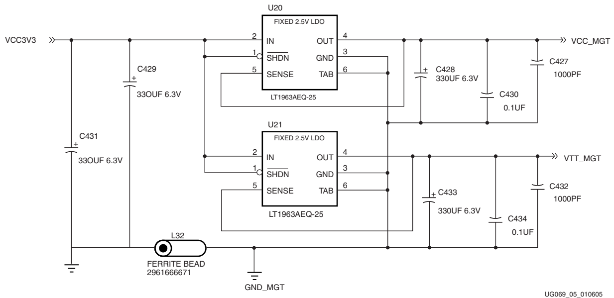
Figure 2-2: MGT Power
