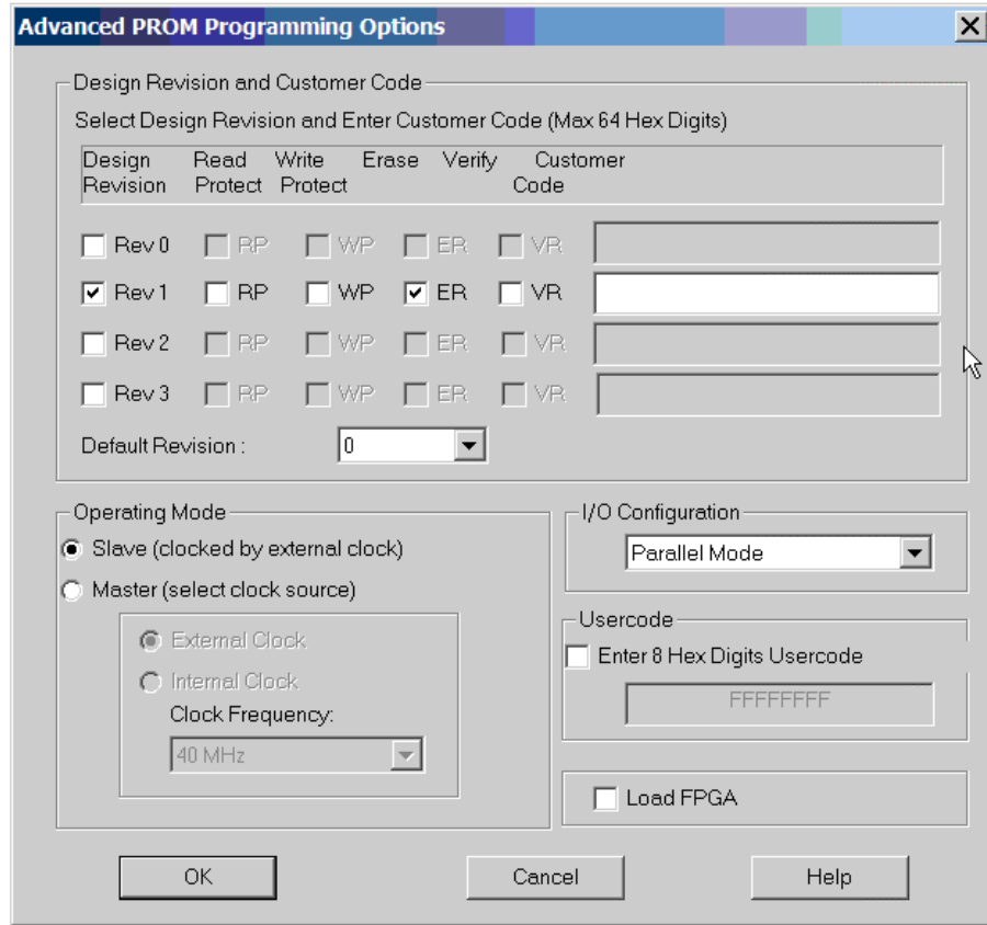
Figure B-14: PROM Programming Options
