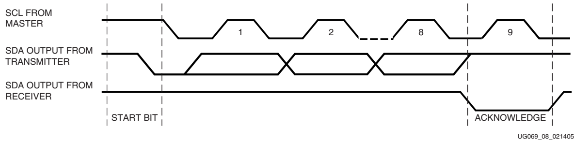
Figure 2-7: Acknowledge Response from Receiver
