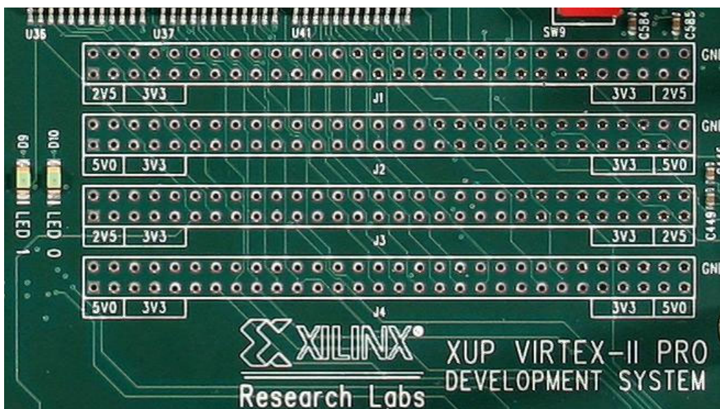
Figure 2-14: Expansion Headers
