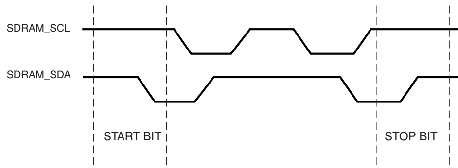
Figure 2-6: Definition of Start and Stop Conditions
