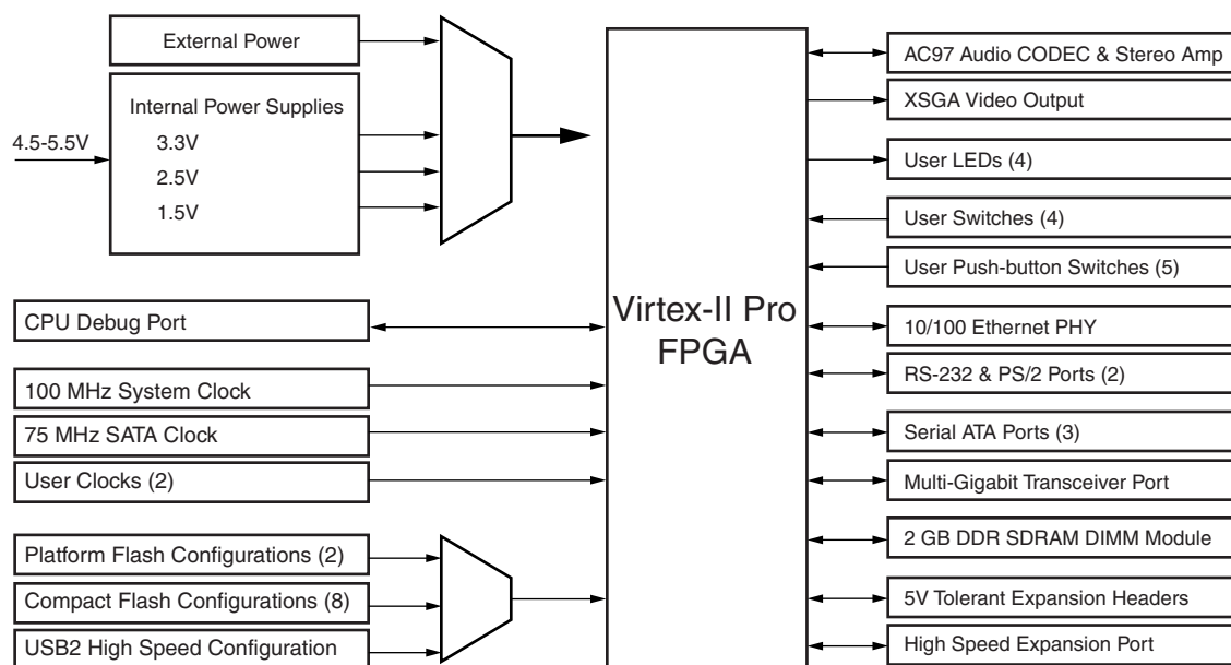
Figure 1-1: XUP Virtex-II Pro Development System Block Diagram
