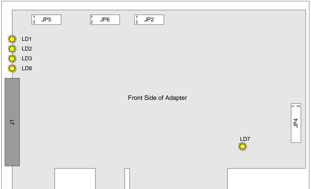
Figure 7 : Connector Locations on the HSS8 PCI and HSS4NG PCI Adapters (FP)
