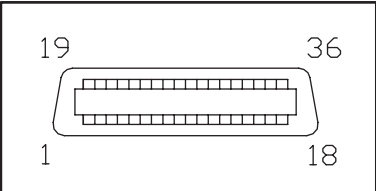
<Centronics Parallel>
