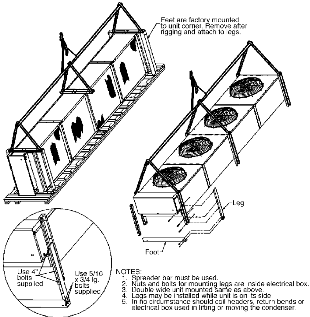
Figure 1. Rigging Instructions.
