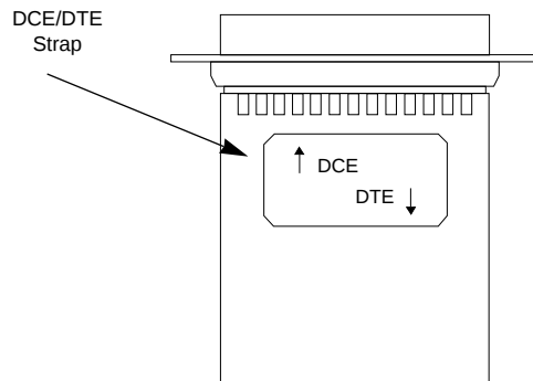
Figure 3. DCE/DTE strap orientation on PC board
