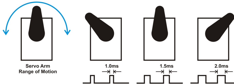
Figure 3-1: RC Servo Arm Travel & PWM Signal
