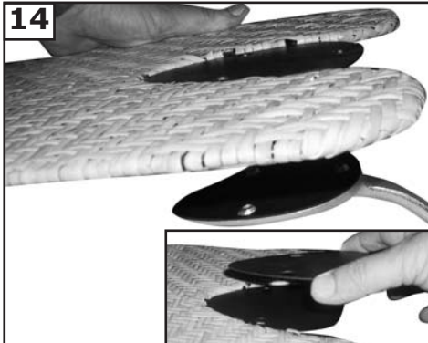
14 Place shim on blade. Place blade onto blade holder.
