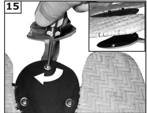
15 Install 3 screws and washers per blade and tighten securely. Repeat for all 5 blades
