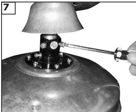
7 Tighten both yoke set screws to further secure downrod.
