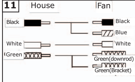
11 For pullchain controls, follow diagram above. Make sure that all exposed wiring is secured inside wire nuts. Note: Wires from house may vary in color and may not include ground wire. After wiring is complete, gently push wires into junction box with wire nuts pointing upward. Refer to point 3 of safety tips.
