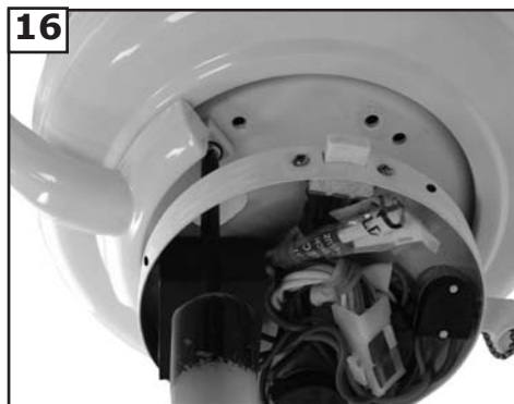
16 Check the motor for plastic shipping stabilizer tabs, and remove them if they are present. Attach blade assembly to motor using the motor screws and washers provided. Tighten screws securely.
