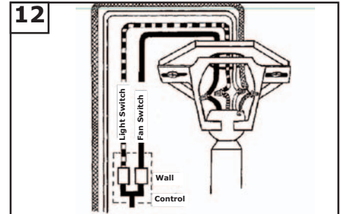
12 For control of fan and optional light from wall location, follow diagram above. NOTE: A professional electrician is recommended for this type of installation.
