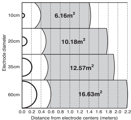
Figure 7. Larger anodes increase the fishing area.
