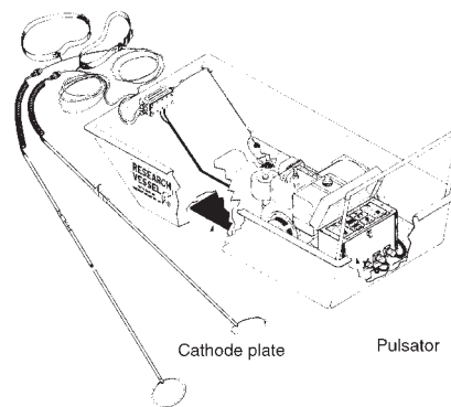
Figure 11. Bottom mounted cathode plate on SR-6.
