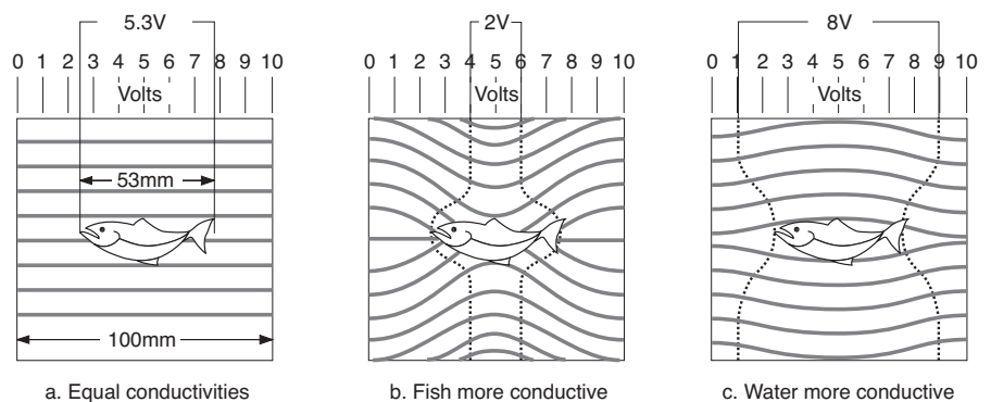
Figure 2. Electric field patterns caused by fish.
