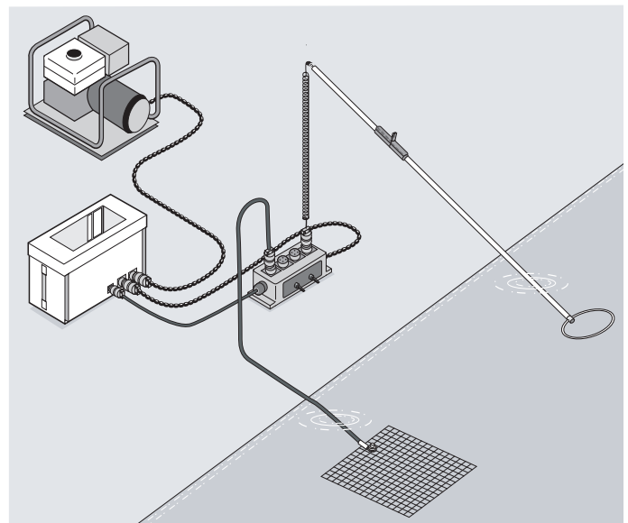
A typical shore hook-up with electrode pole and control box.
