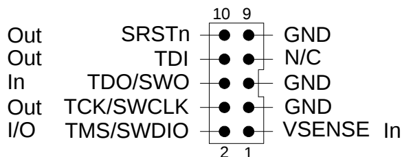
Figure 2-6. JTAG/SWD Connector J1
