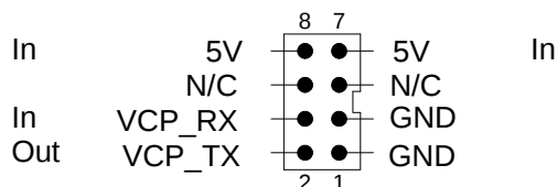
Figure 2-4. PWR/UART Connector
