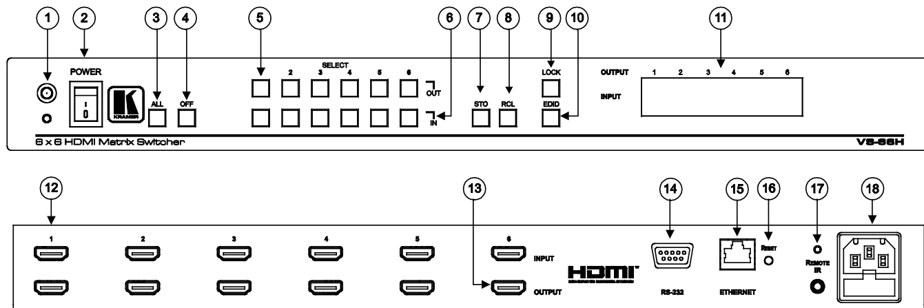
Figure 1: VS-66H 6x6 HDMI Matrix Switcher
