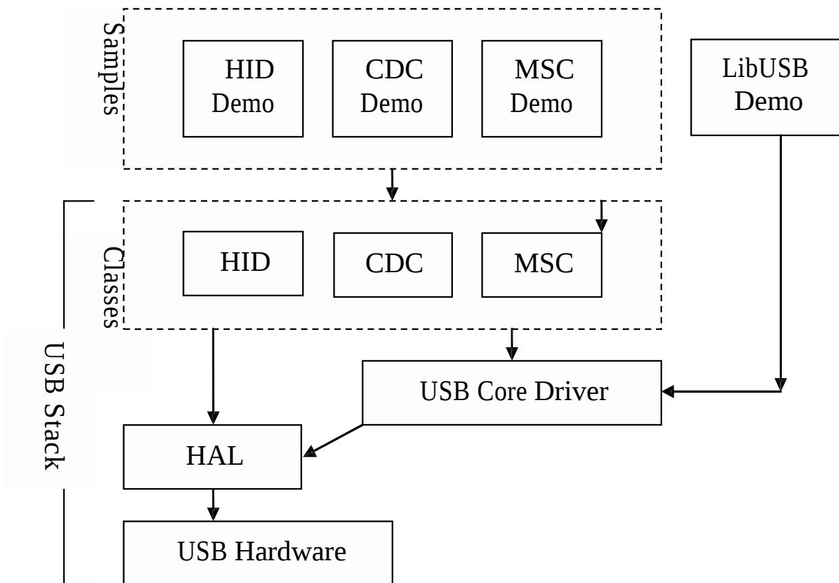
Figure 1 - Embedded SW, including Layers of USB Stack
