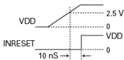
Figure 3 Reset Timing
