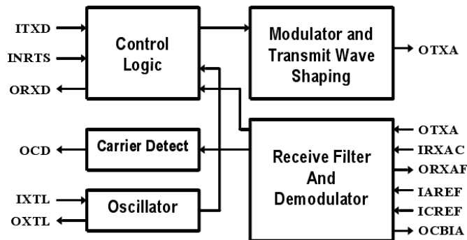
Figure 4 HT1200M Block Diagram
