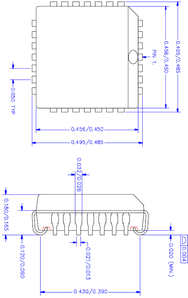
Figure 11 PLCC28
