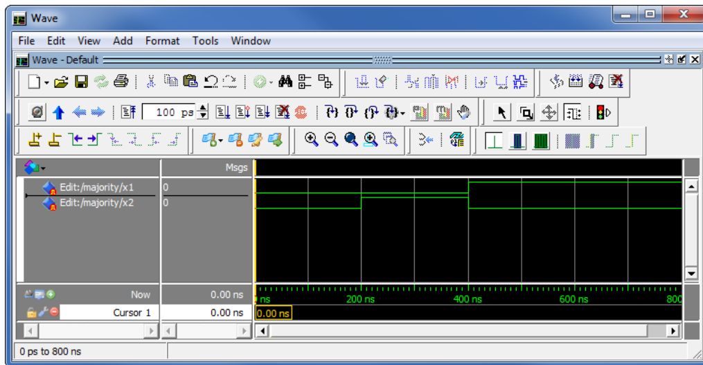
Figure 18. The modified waveform.
