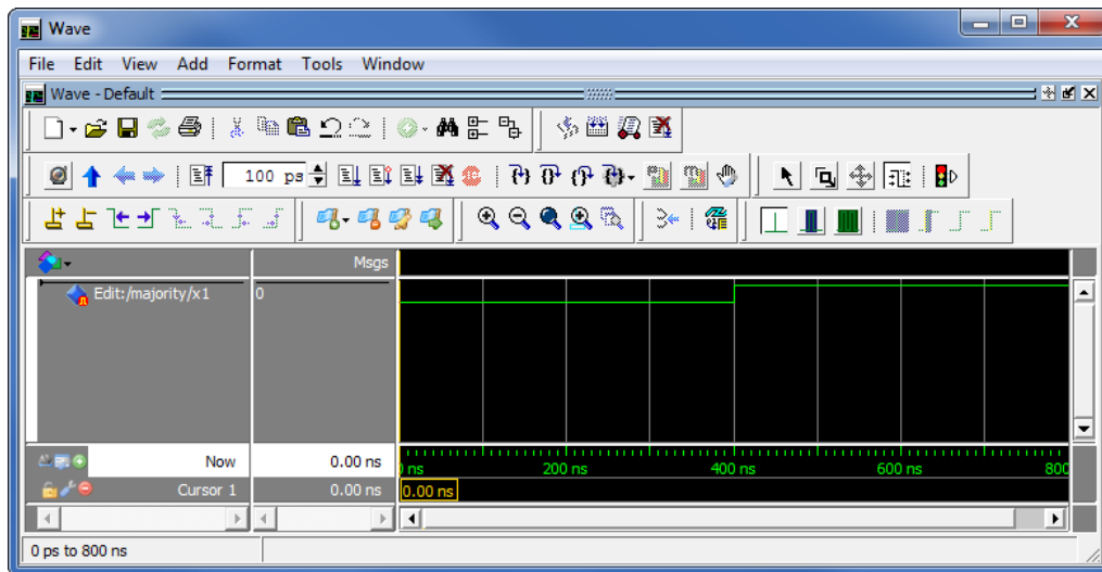
Figure 14. The completed waveform for x_1 input.
