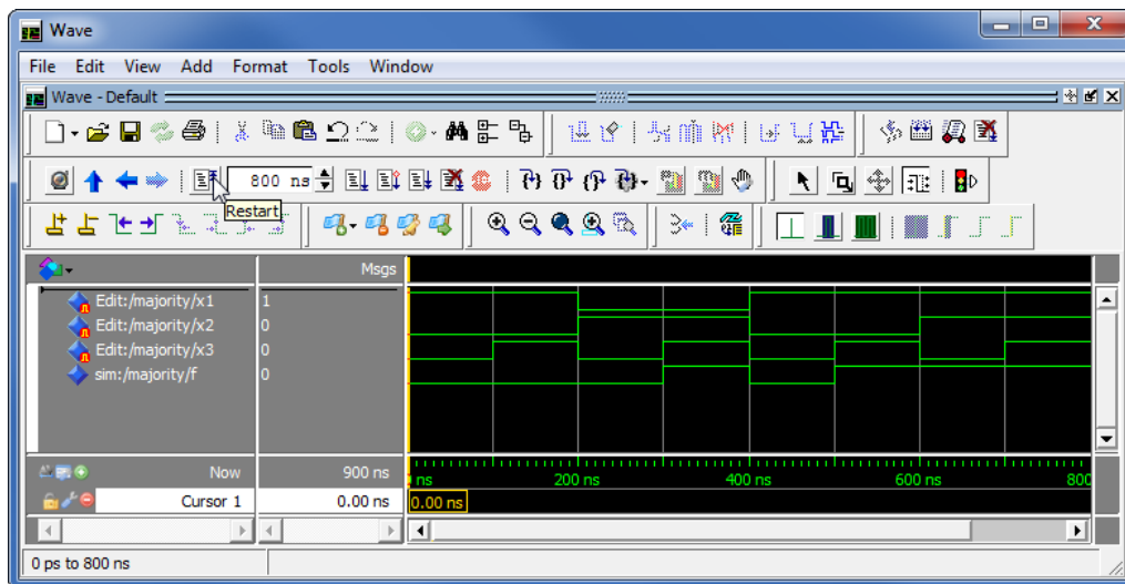
Figure 28. Changed input waveforms.
