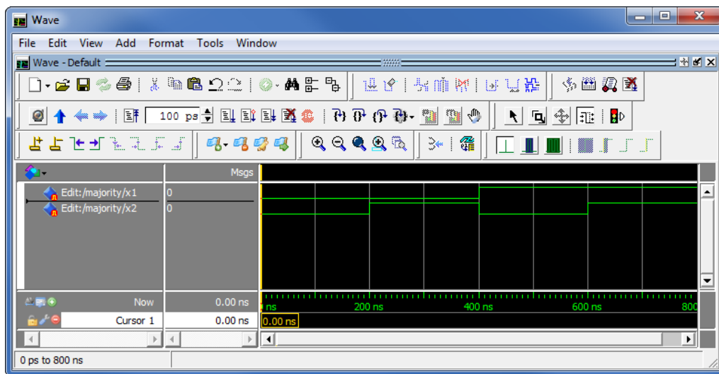
Figure 19. Completed waveforms for x_1 and x_2 .
