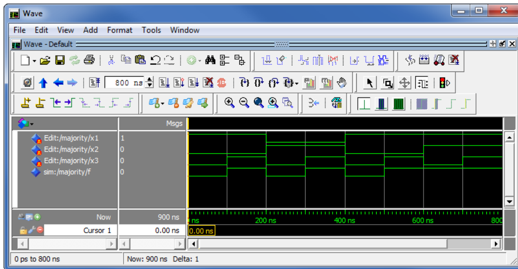
Figure 30. Result of the new simulation.
