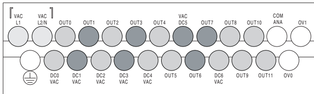
Output Terminal Block
