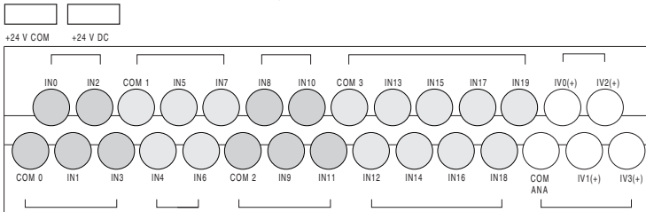
Input Terminal Block
