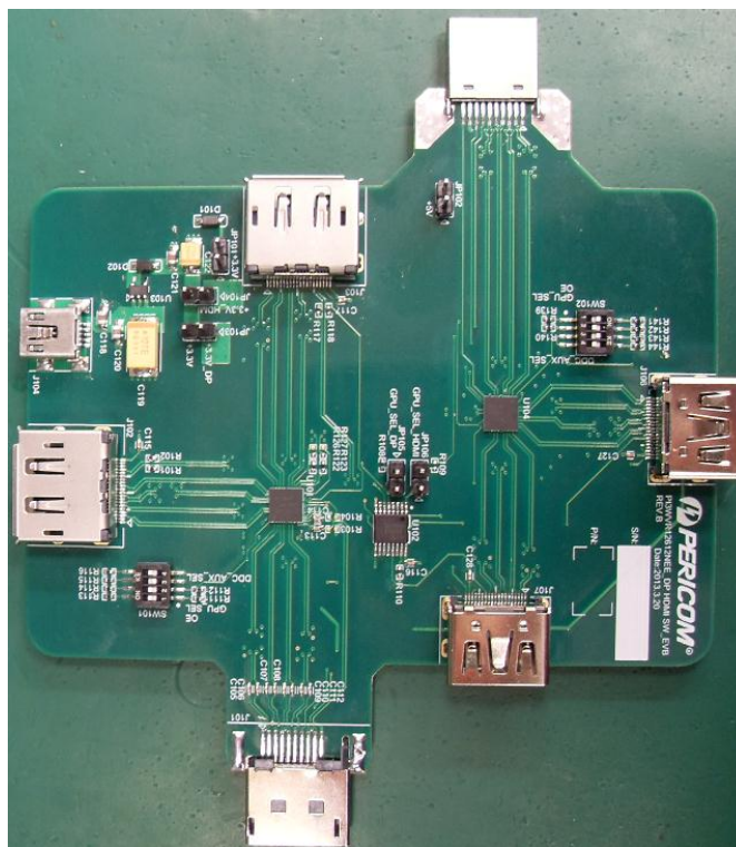
Figure 3: Top View of PI3WVR12612NEE Demo Board Rev.B
