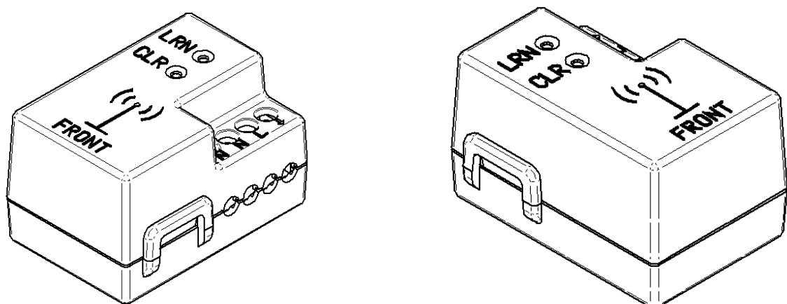
Figure 2: RCM 250 housing
