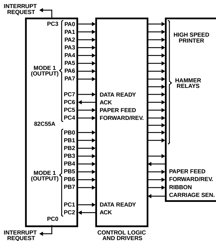
FIGURE 18. PRINTER INTERFACE
