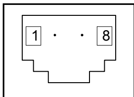
RJ-45
