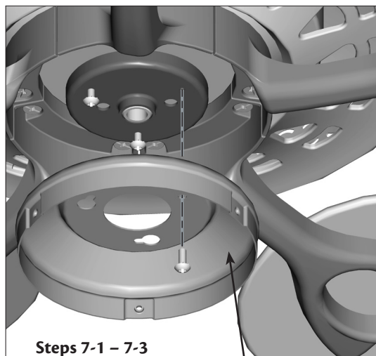
Housing Assembly Screw
