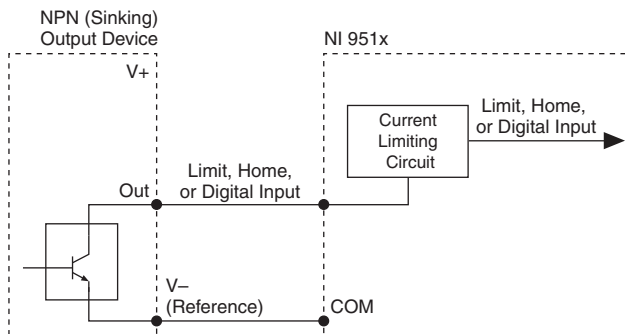
Figure 3-7. Limit Input Configured for Sourcing
