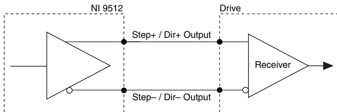
Figure 3-2. Differential Step and Direction Output Connection
