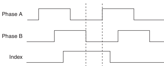
Figure 3-10. Incremental Encoder Phasing Diagram
