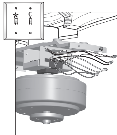
Wire Connector
