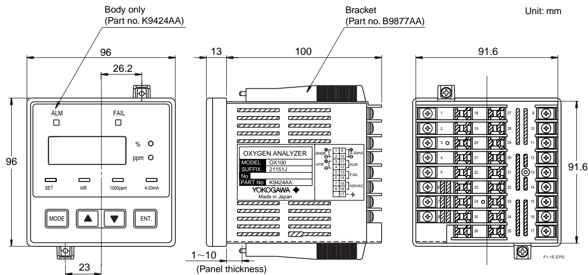
Fig. 1.1 External Dimensions of Instrument
