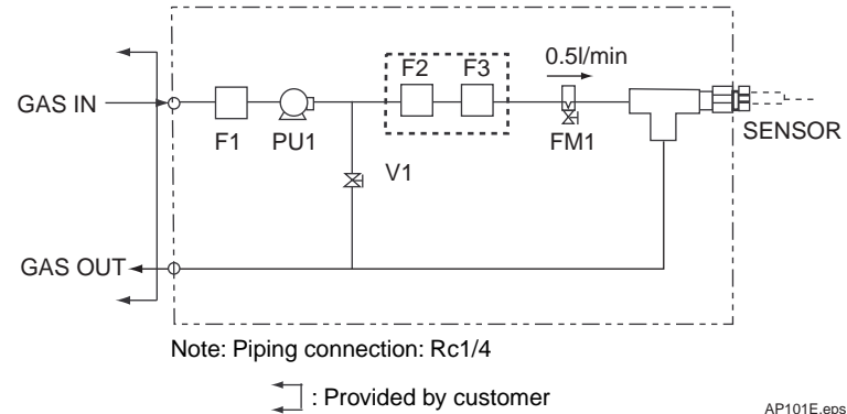
Figure1. Piping Diagram
