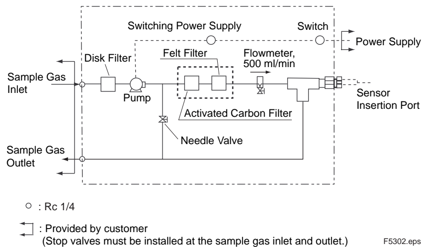
Figure 2.8 Sampling Unit (K9424GA, Optional)
