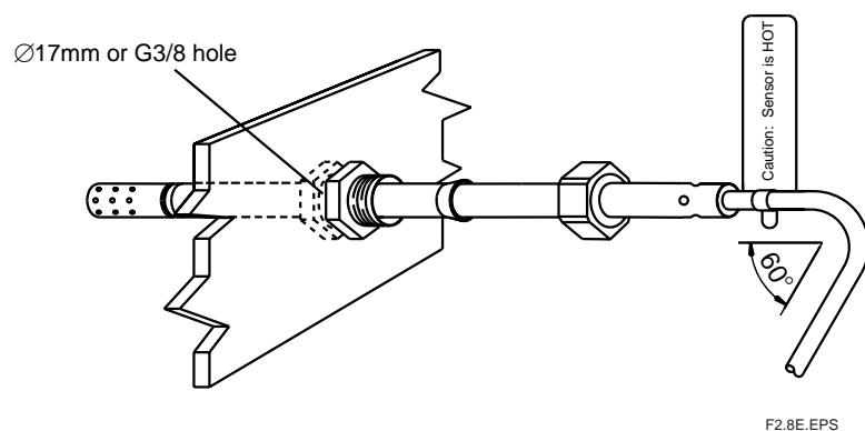
Figure 2.8 Installation of Sensor
