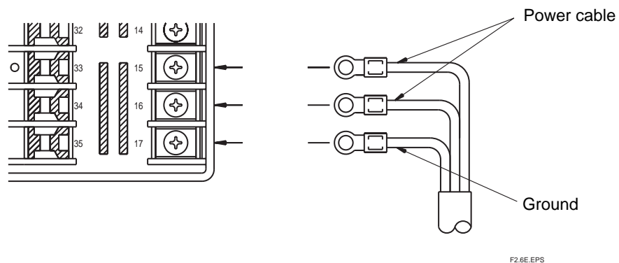
Figure 2.6 Power wiring
