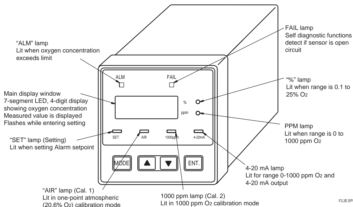
Fig. 2.2 Display panel
