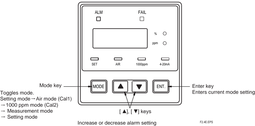
Figure 2.4 Operation Keys
