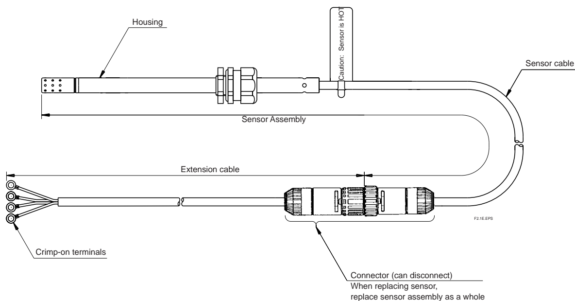
Figure 2.1 Oxygen sensor
