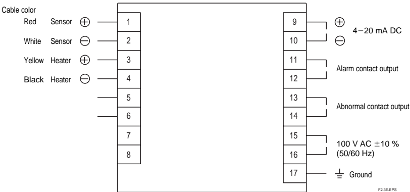
Figure 2.3 Terminal layout
