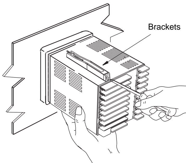
Figure 2.5 Mounting
