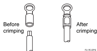
Fig. 2.7 Crimp-on terminals
