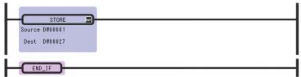
Fig. 2.3 Program Sample
