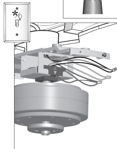
Wire Connector
