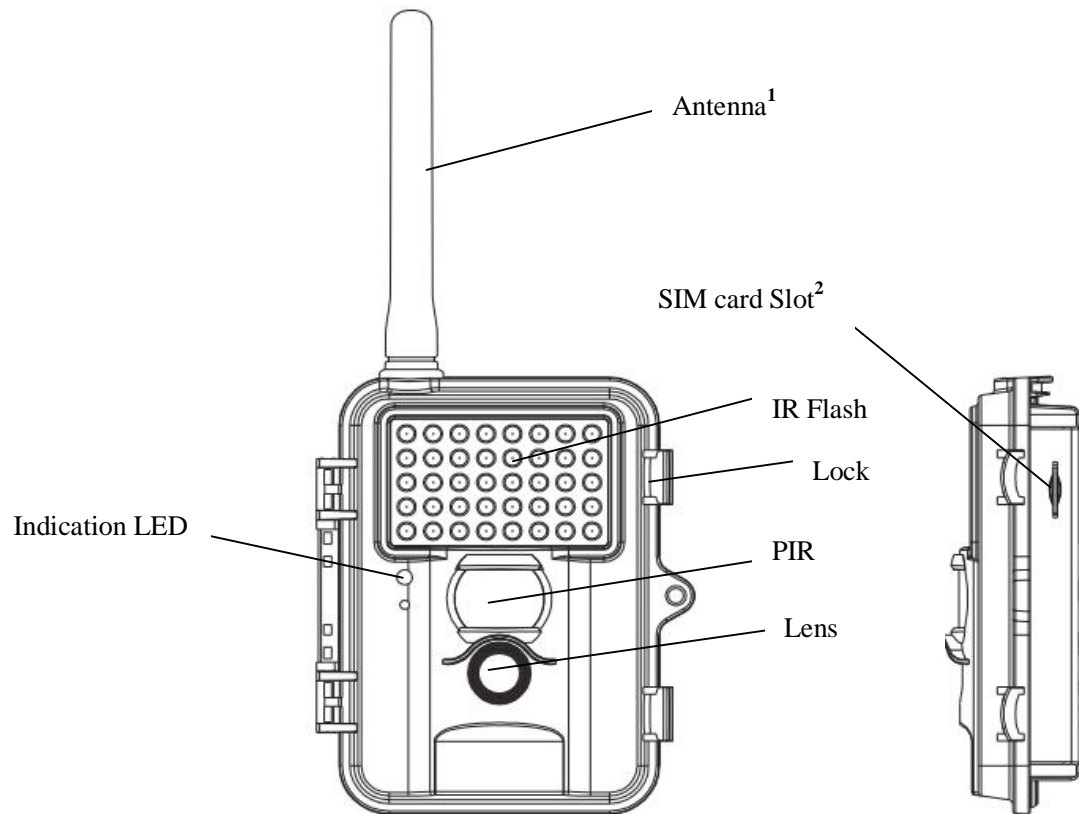
Figure 1: Front View
