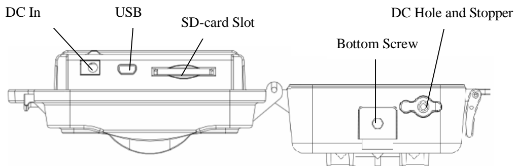
Figure 3: Bottom view
