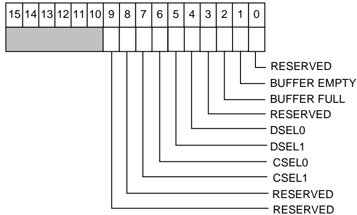
Fig. 4.22: Status Register 2
