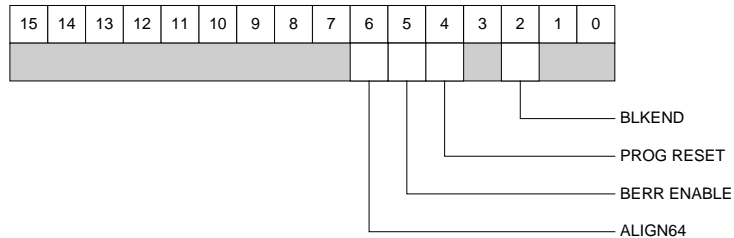
Fig. 4.17: Control Register 1
