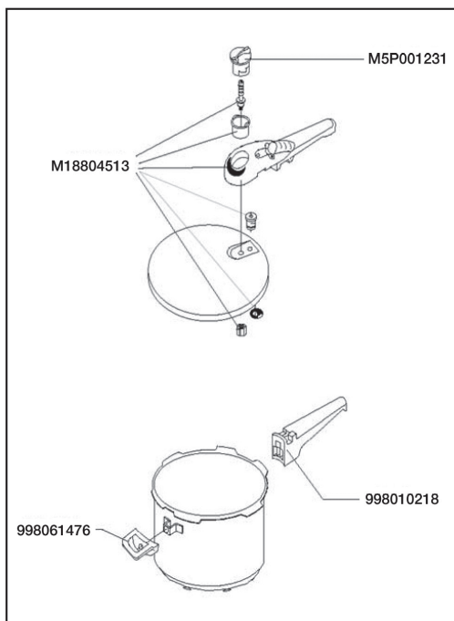
998061476 Helper Handle
