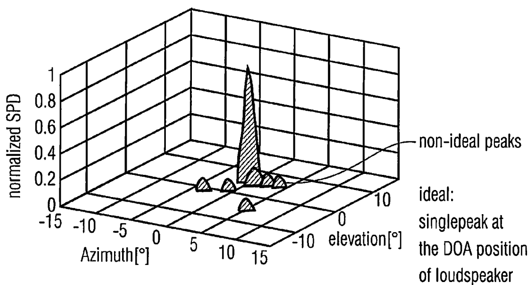
Observed spatial power density ( \Gamma ) of a loudspeaker placed in [\varphi, \theta] = [0^\circ, 0^\circ]
