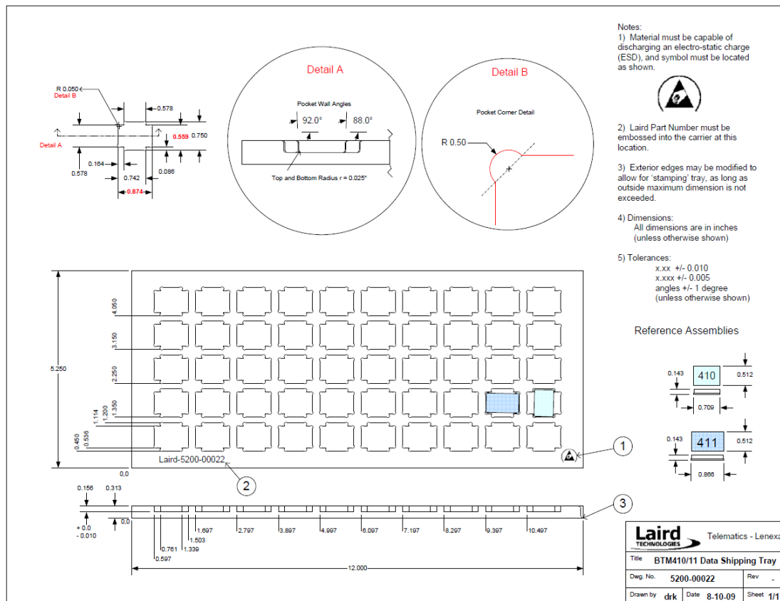
Figure 8: BTM44x Shipping Tray Details
