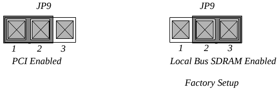
Figure 2-7. JP9 - Local Bus Mode
