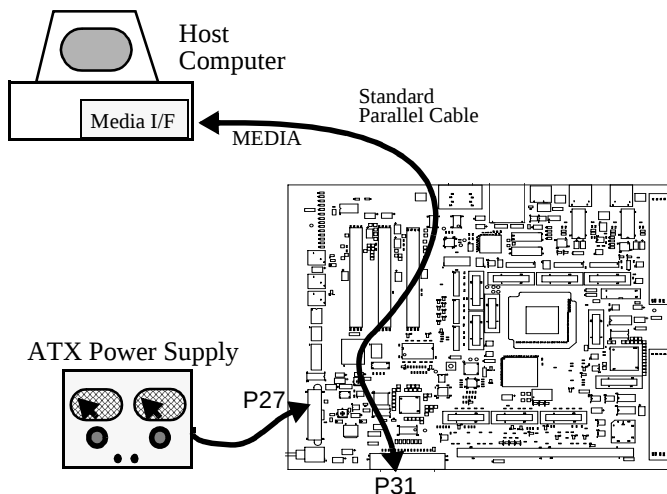
Figure 2-13. Host Controlled Operation Scheme - Parallel Port
