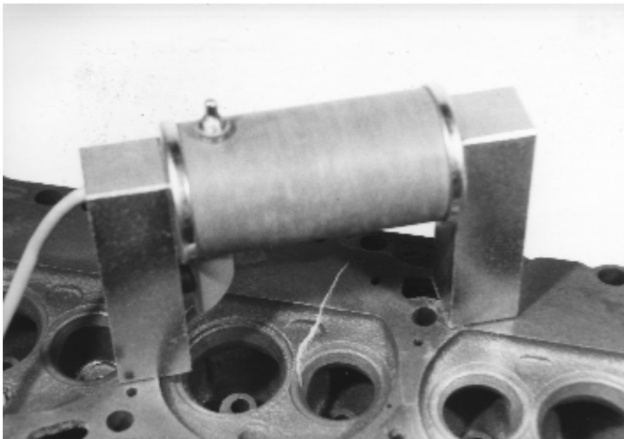
Electro Magnet positioned over crack
