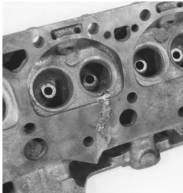
Remove Excess Plug Material
