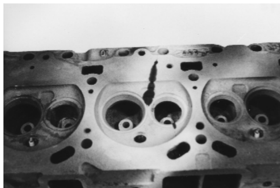
Crack Identified by Kwik-Chek
