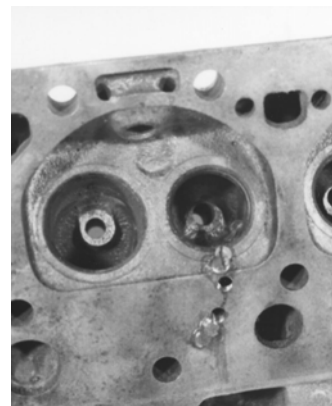
Continue to Fill in with Plugs
