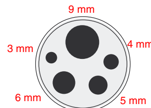
Multi-hole M01 (MTC-320 A) (MTC-650 A)
