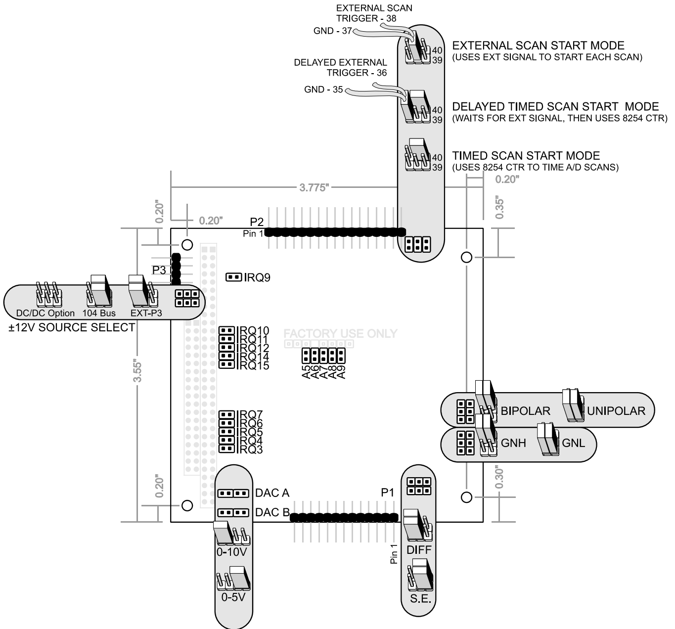
Figure 3-1: Option Selection Map
