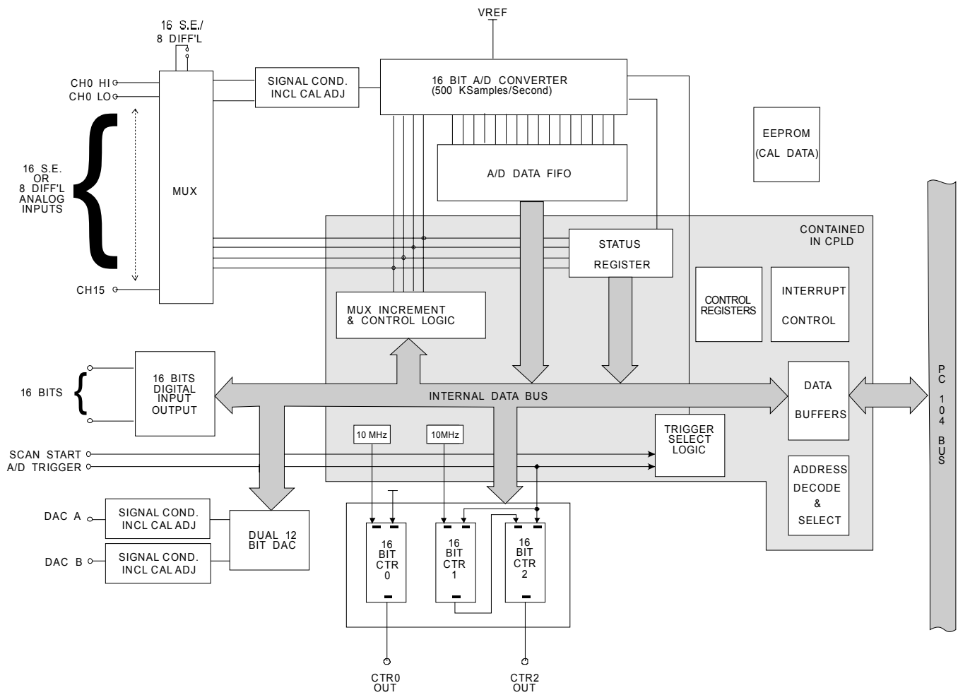
Figure 1-1: Block Diagram
