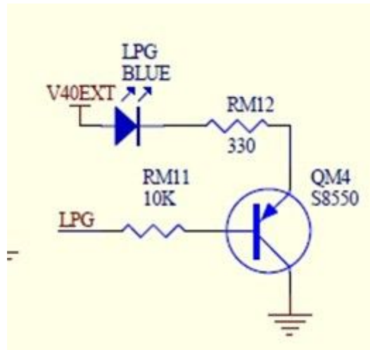
Figure 3-12 LPG reference design
