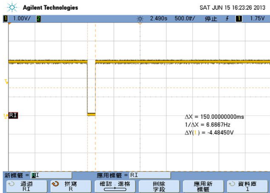
Figure 3-8 The Module gets a message
