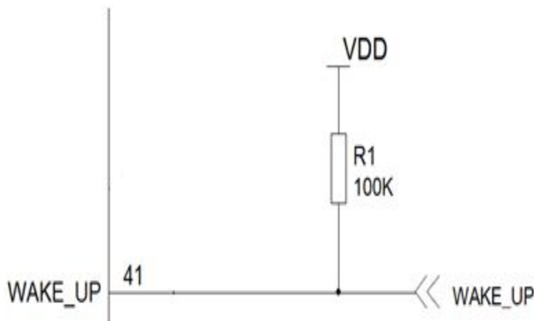
Figure 3-13 Recommended circuit for WAKE_UP
