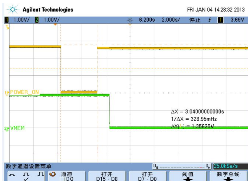
Figure 3-4 Power off succeed
