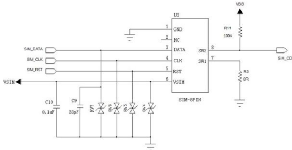
Figure 3-10 SIM card reference design
