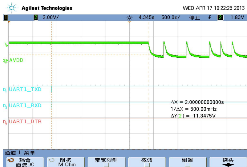
Figure 3-6 ats24=2 , set module to sleep mode after 2s
