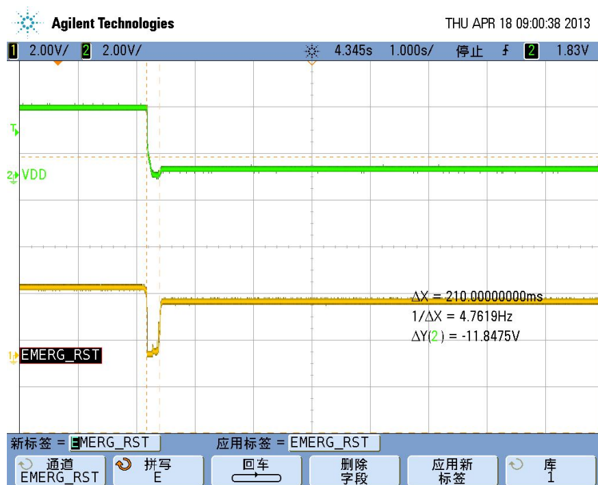
Figure 3- 11 EMERG_RST pull low, G510 reset peremptorily
