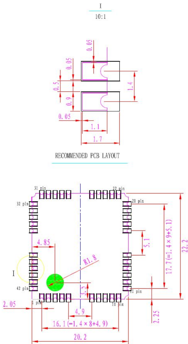
Figure 5-2 Recommended PCB layout (Top View)
