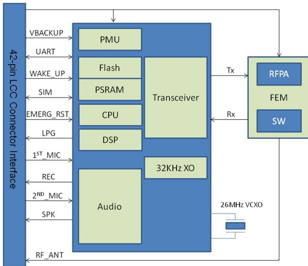
Figure 3- 1G510 Block Diagram
