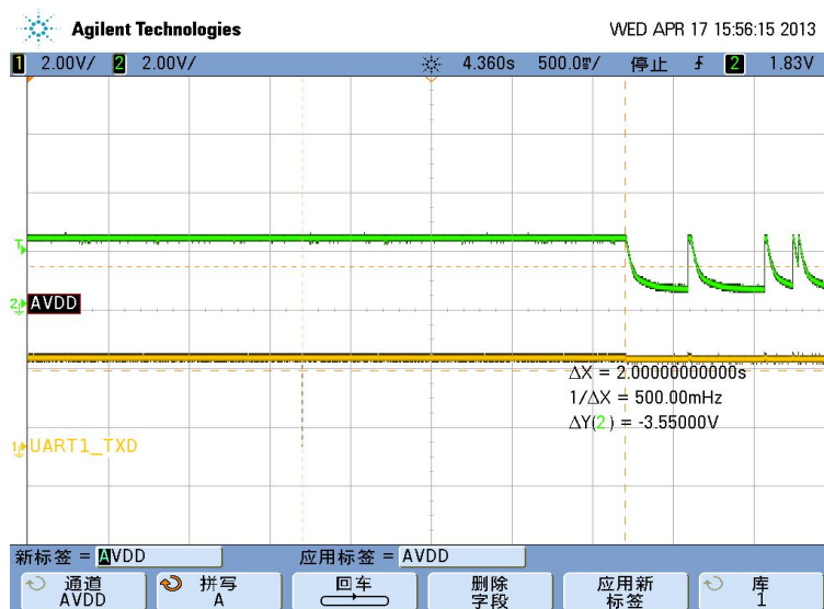
Figure 3-5 ats24=2, set module to sleep Mode after 2s
