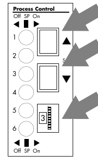
Figure 4-23 Electrometer Module Showing Setpoint Set Buttons and Channel Select Thumbwheel
