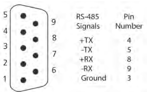
Figure 3-14 RS-485 Connector
