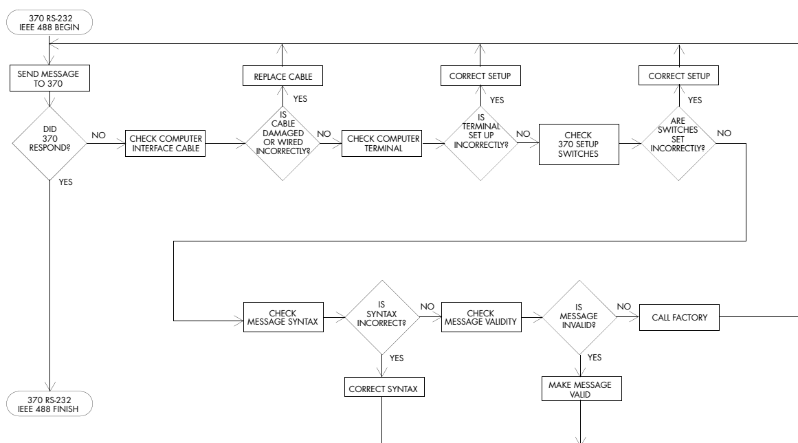
Figure 7-11 RS-232/IEEE 488 Interface
