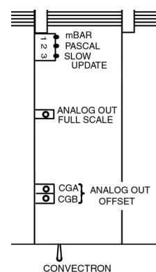
Figure 4-18 Top View of Convection Gauge Module Showing Analog Output Offset Adjustment
