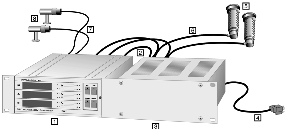
Figure 1-1 Stabil-Ion Vacuum Measuring System
