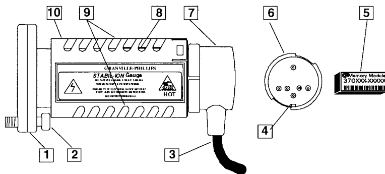
Figure 1-2 Stabil-Ion Gauge
