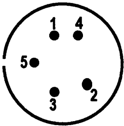
Figure 7-3 Convectron Gauge Base
