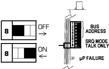
Figure 2-17 Top View of IEEE 488 Module
