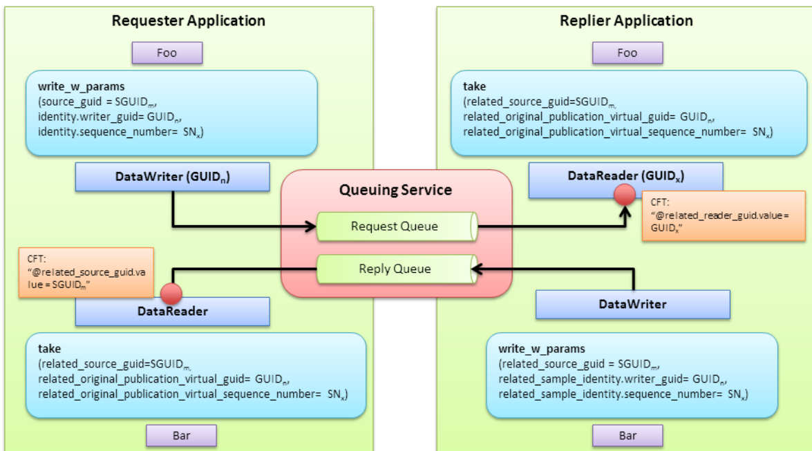
Figure 2.6 Request Generation
