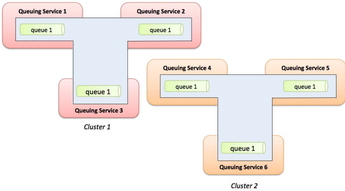
Figure 7.4 Replication Cluster
