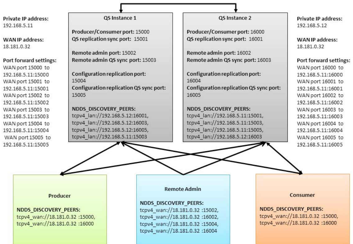
Figure 9.2 Asymmetric TCP Configuration With Replication
