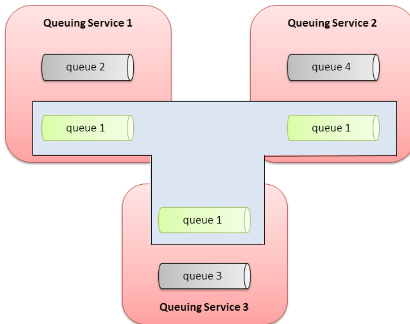
Figure 7.1 Replicating SharedReaderQueues
