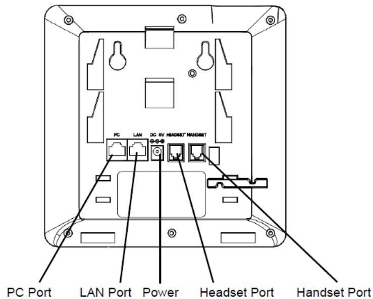
Figure 1: GXP1400/GXP1405 Ports
