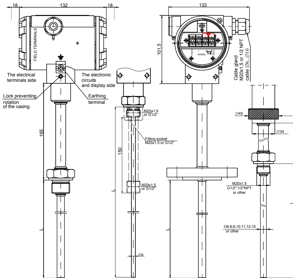
Fig.3. APT-2000ALW smart temperature transmitter.
