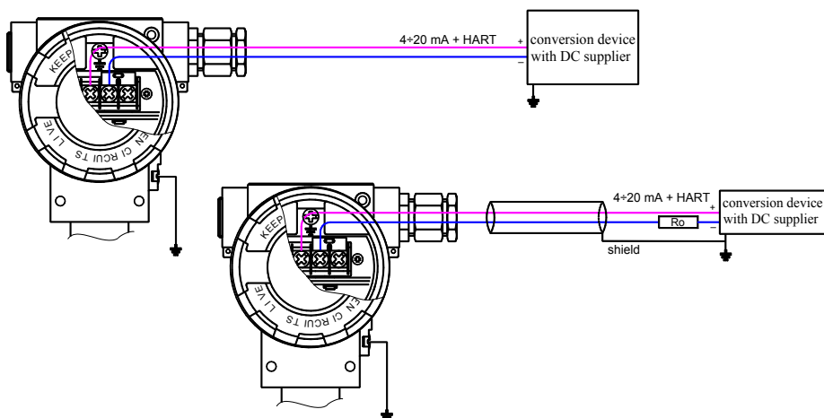
Fig. 1b. APT-2000ALW temperature transmitter for MID application. Recommended by manufacturer way of earthing to the measuring system.
