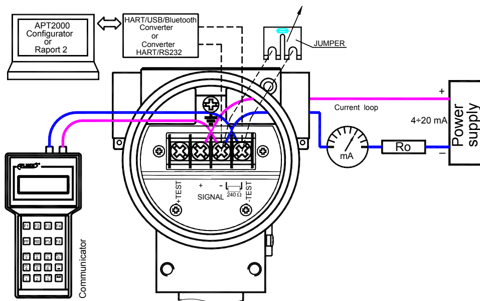
Fig.2d. The link of transmitter and communicator or converter to <TEST-> <SIGNAL-> transmitter terminals in case of the resistance in current loop is smaller than 240Ω .
