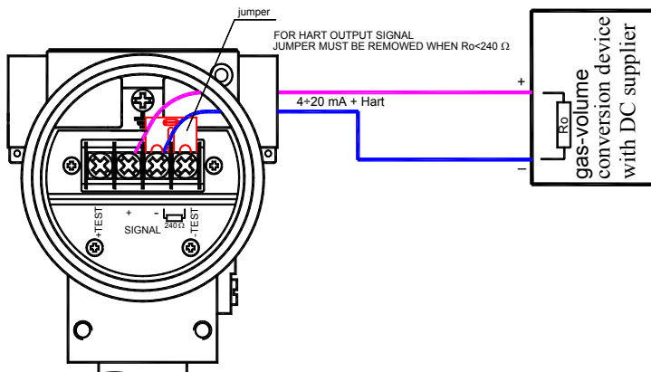
Fig. 1a. APT-2000ALW for MID application. Connecting diagram of transmitter to powering and measuring installation.
