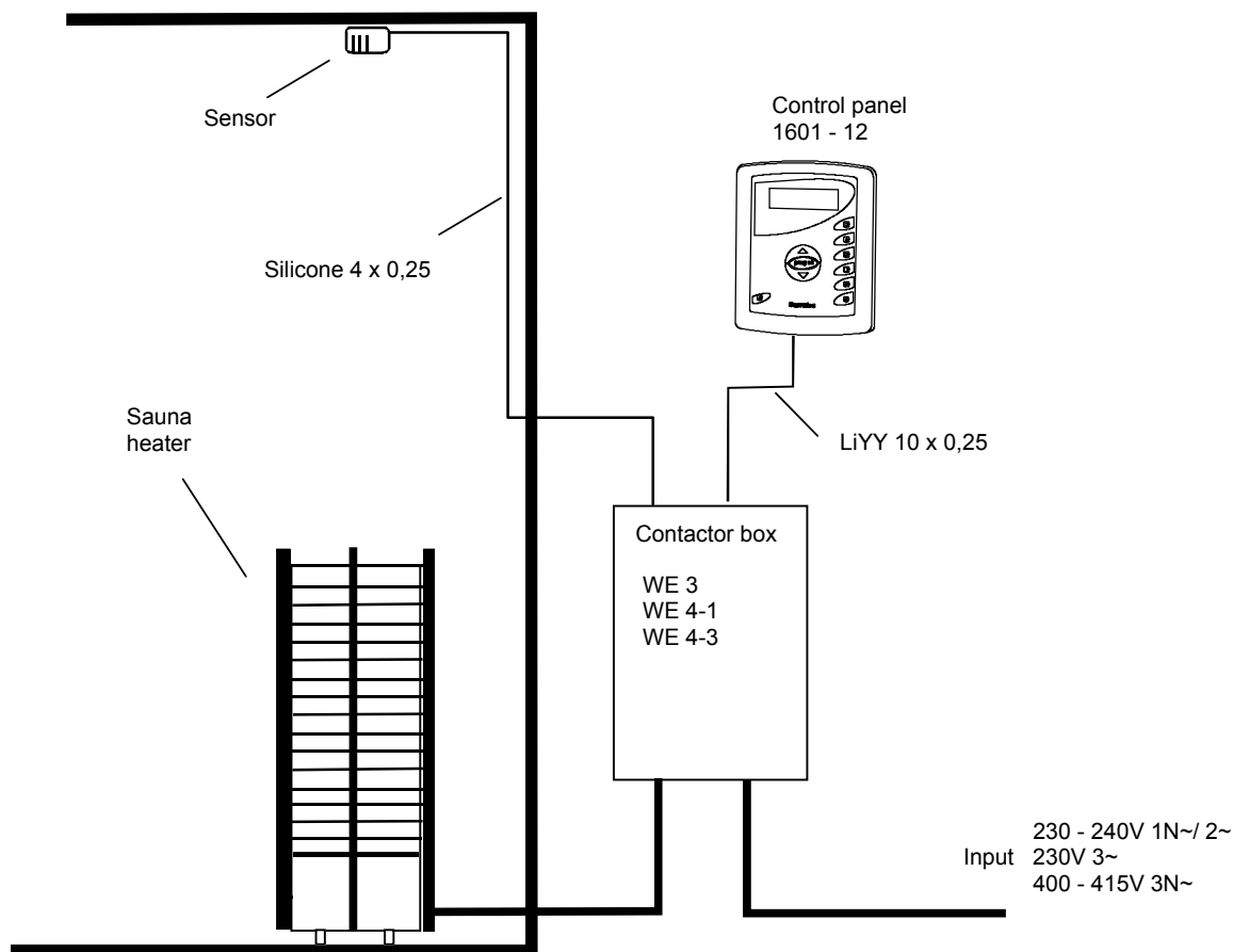
Image 3 Principle image
