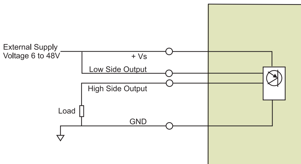
Figure 6 : Output Wiring as High Side Switch
