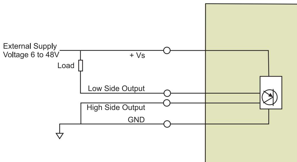
Figure 7-1 : Output Wiring as Low Side Switch
