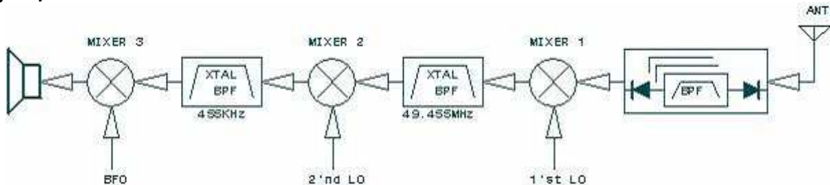
< ↑ RX BLOCK DIAGRAM >
