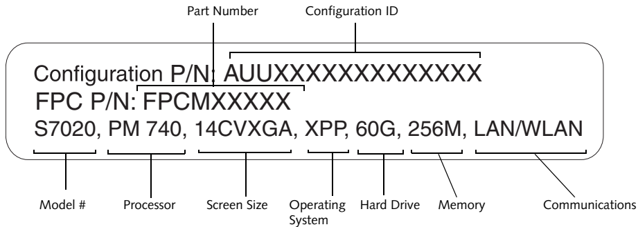
Figure 7-1 Configuration Label
