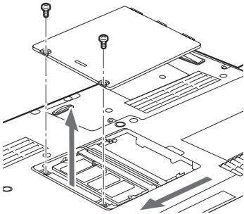
Figure 4-9. Opening the Memory Upgrade Compartment
