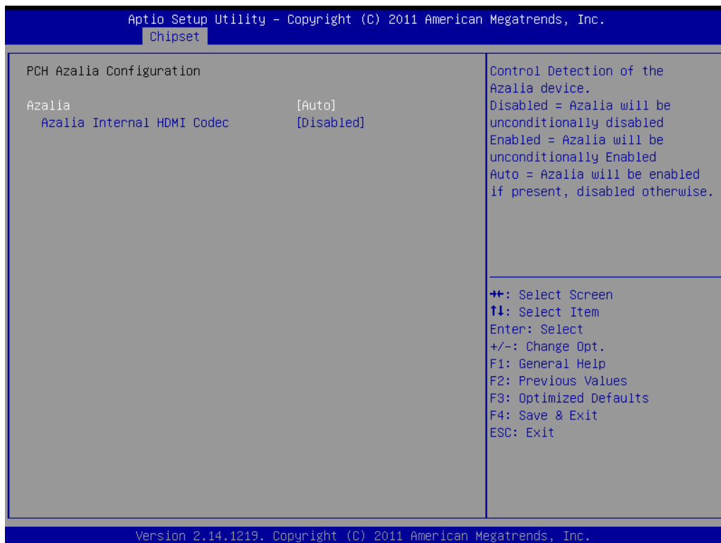
Figure 3.39 PCH Azalia Configuration
