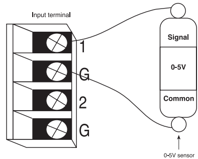
0-5V sensor
