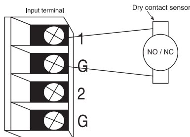
Dry Contact
