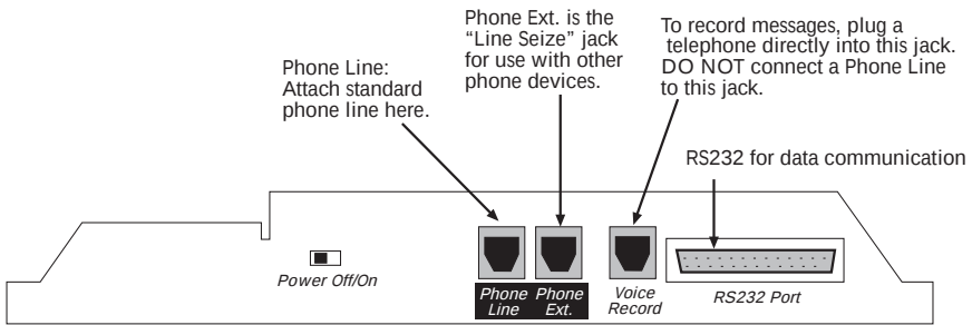
CPP Monitor 2000—Front View
