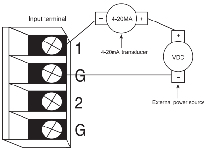
4-20mA Transducer
