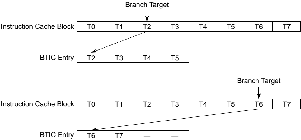
Figure 4. Alignment of Target Instructions in the BTIC
