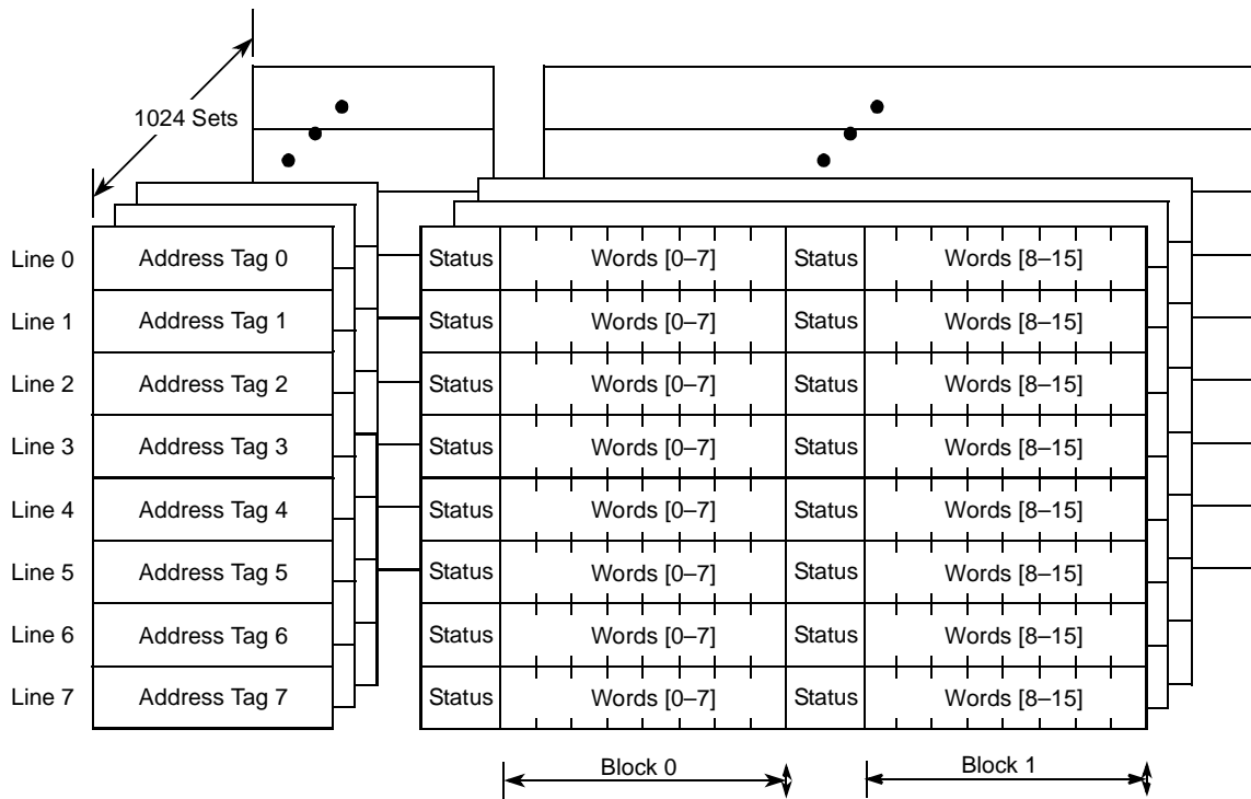
Figure 6. L2 Cache Organization for the MPC7447, MPC7457, MPC7447A, and MPC7448
