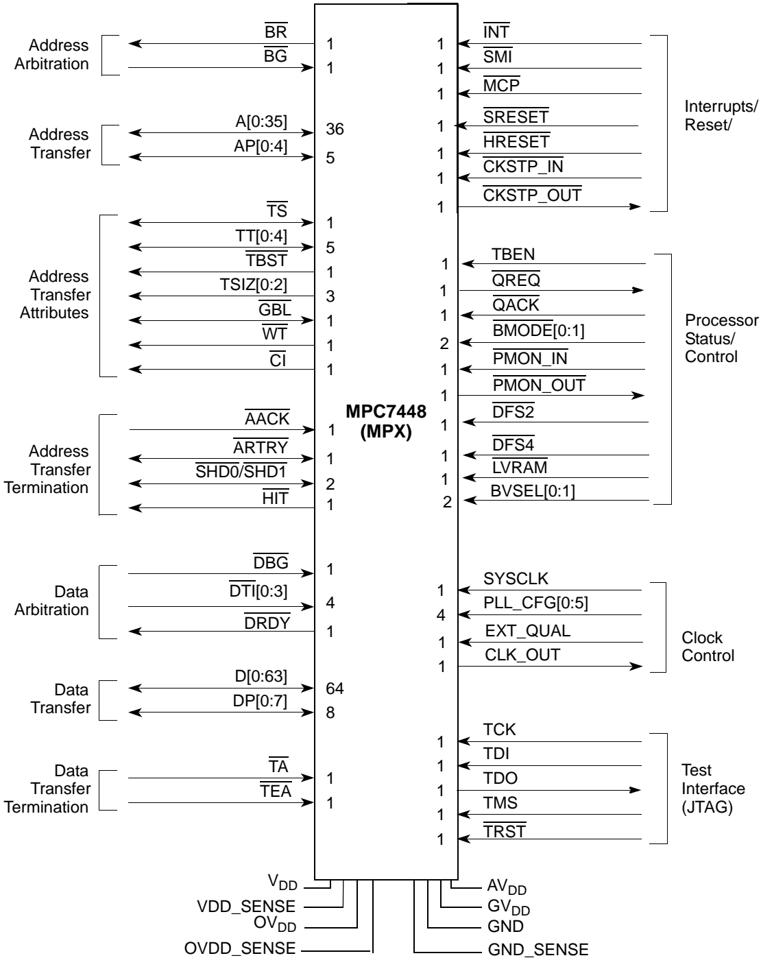
Figure 10. MPX Bus Signal Groups in the MPC7448
