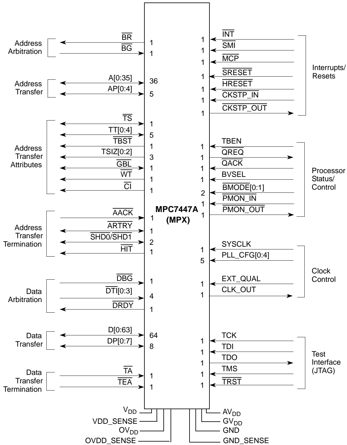
Figure 9. MPX Bus Signal Groups in the MPC7447A
