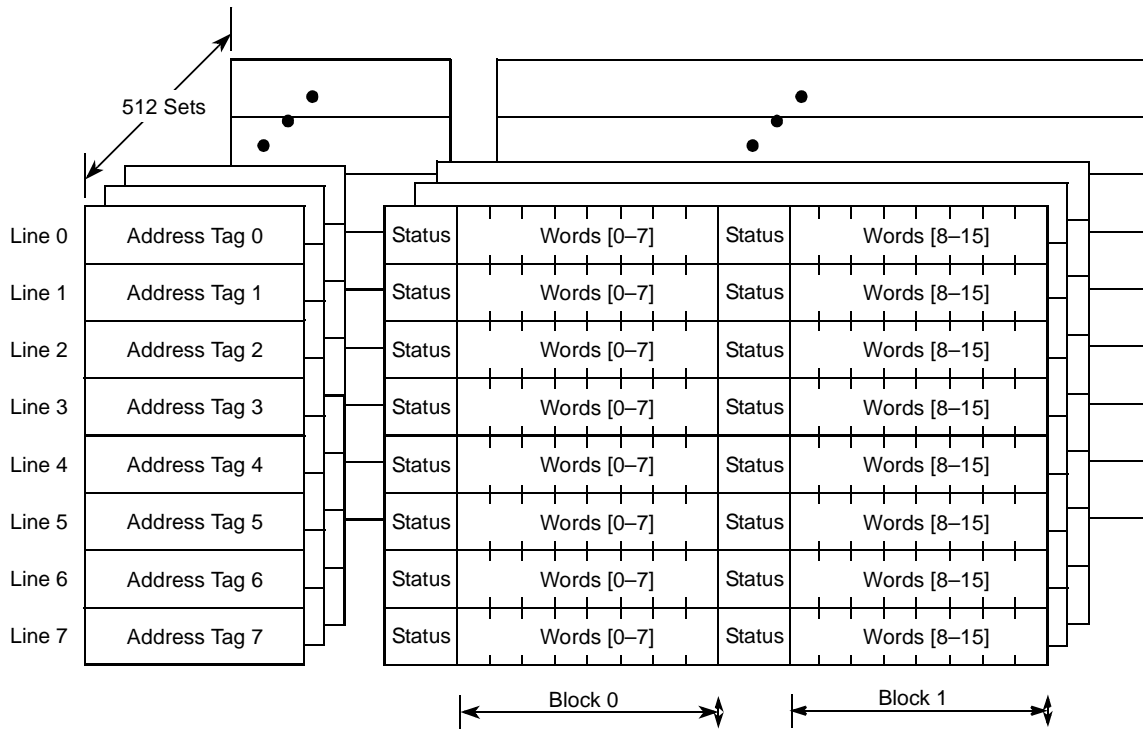
Figure 5. L2 Cache Organization for MPC7450
