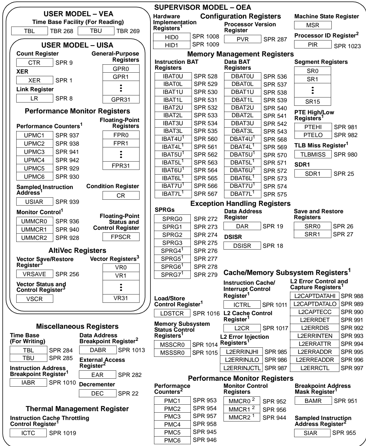
Figure 13 shows the MPC7448 register set.
