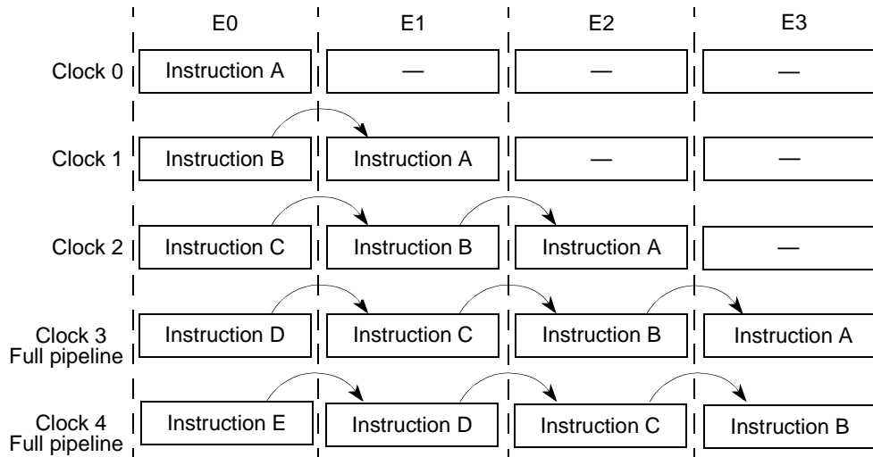
Figure 14. Pipelined Execution Unit
