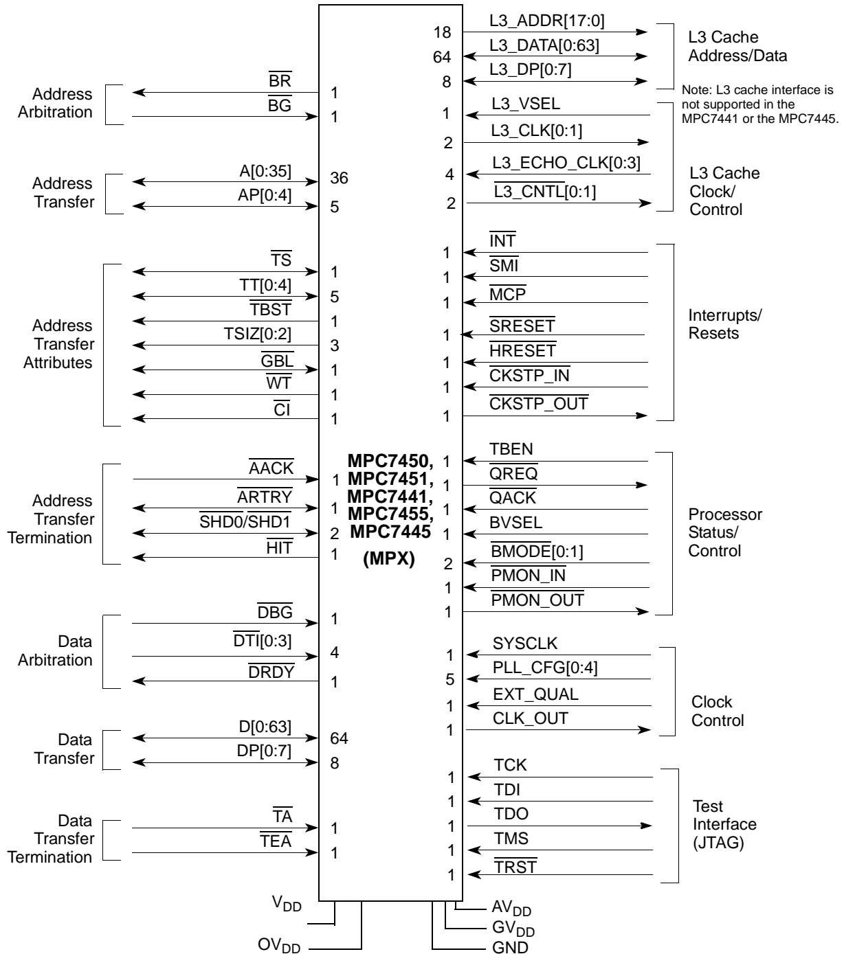
Figure 7. MPX Bus Signal Groups in the MPC7450, MPC7451, MPC7441, MPC7455, and MPC7445
