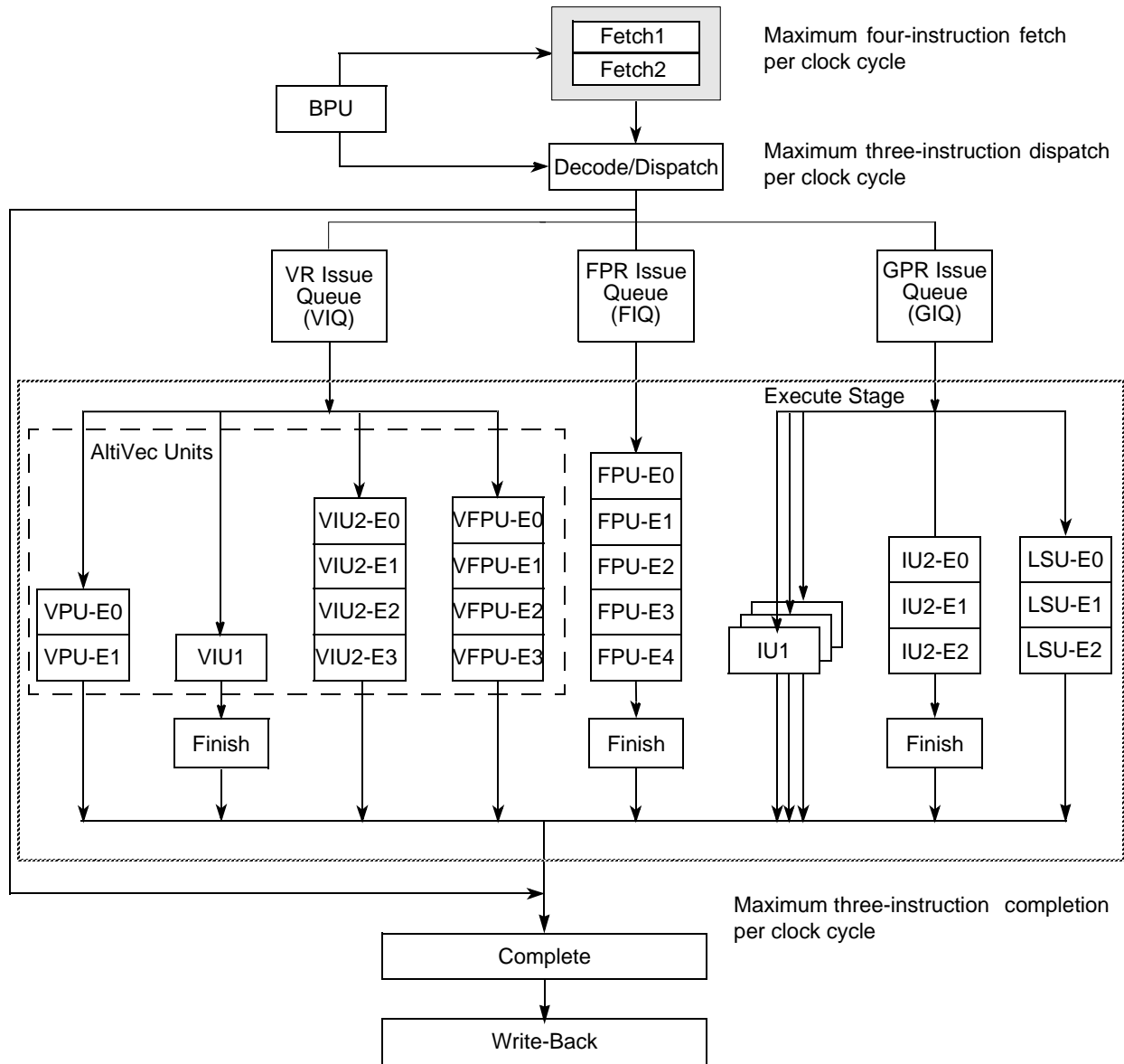
Figure 15. Superscalar/Pipeline Diagram
