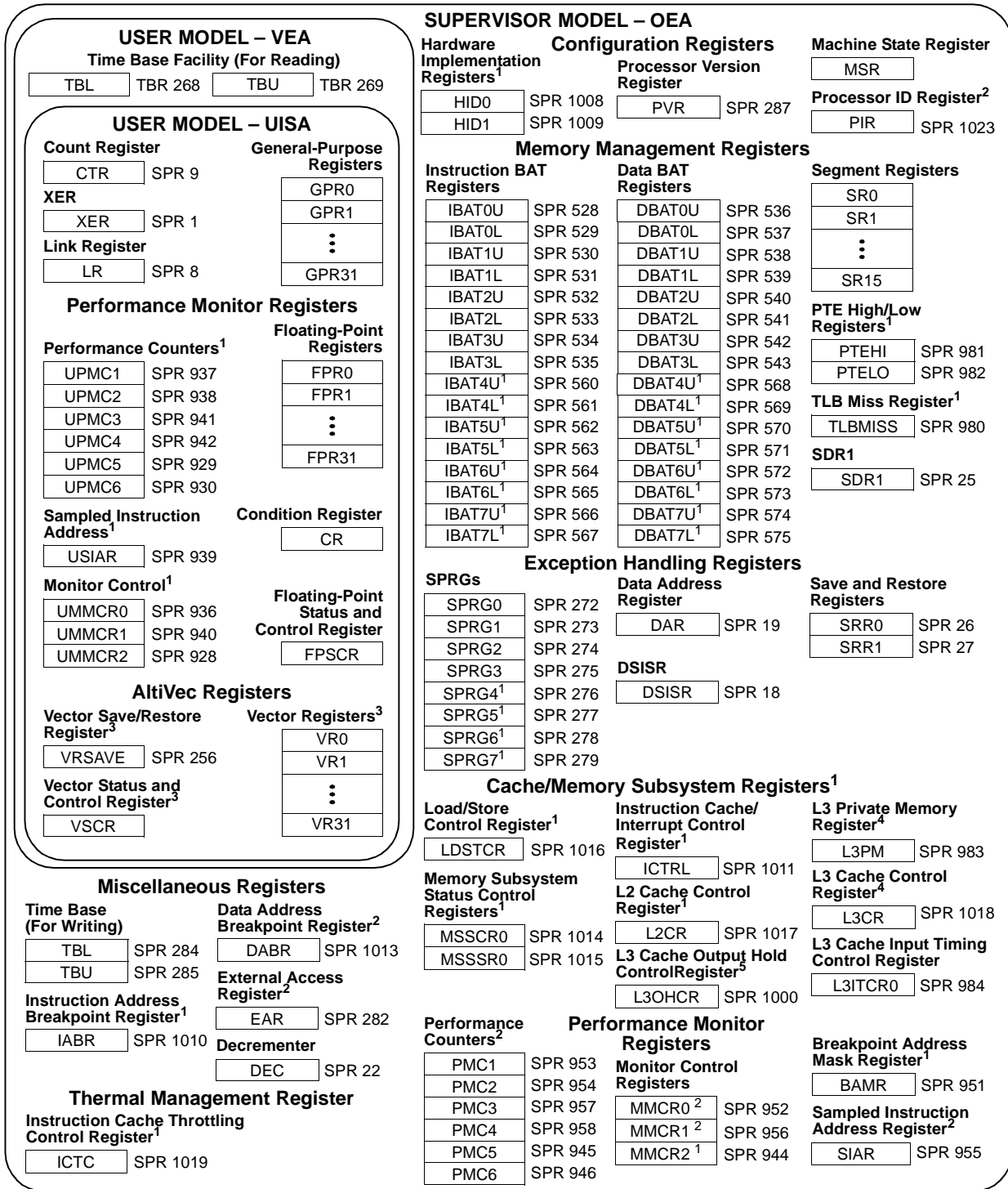
Figure 12 shows the MPC7445, MPC7455, MPC7447, MPC7457, and MPC7447A register set.
