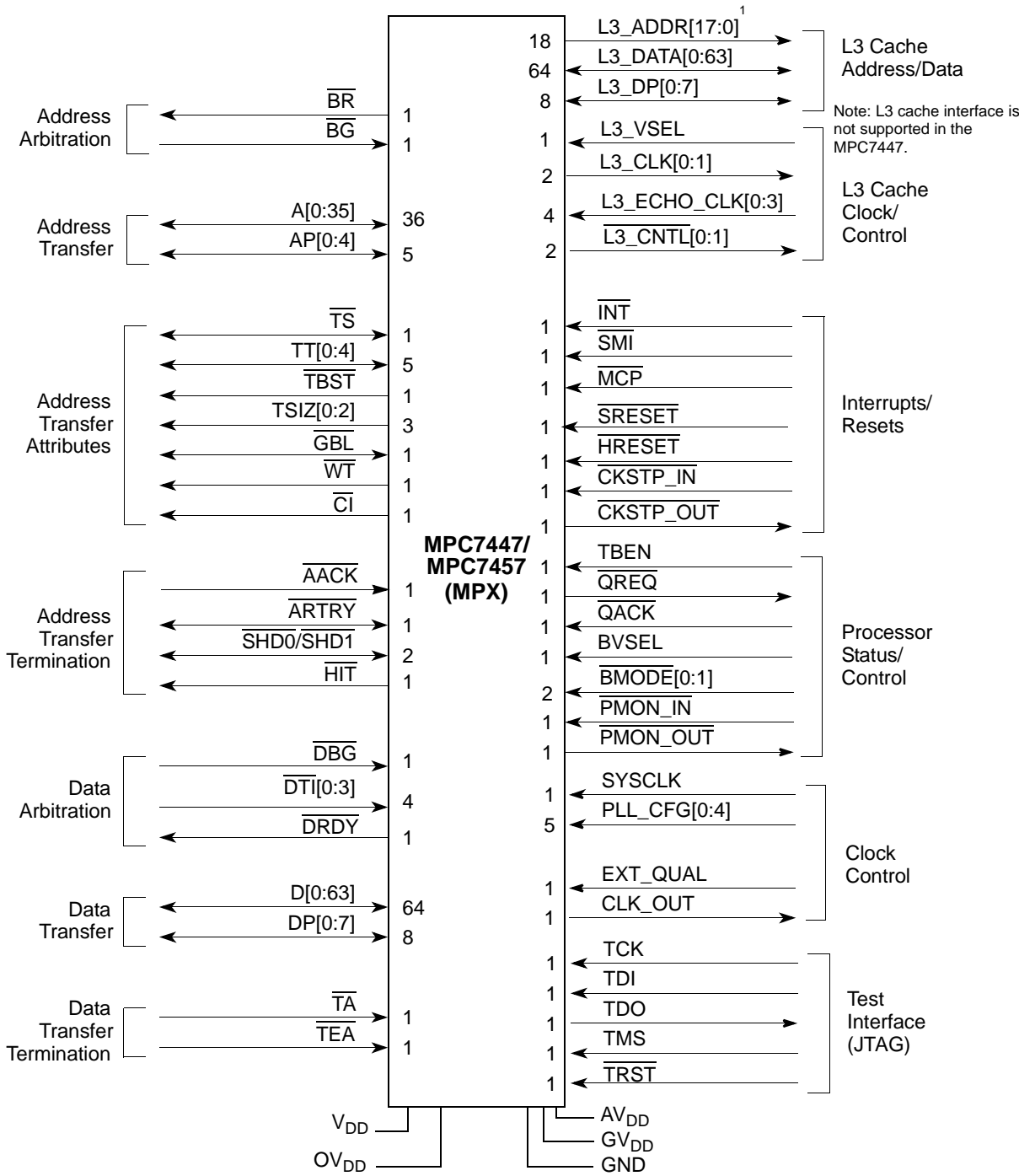
Figure 8 illustrates the signal configuration in MPX bus mode for the MPC7447 and the MPC7457.
