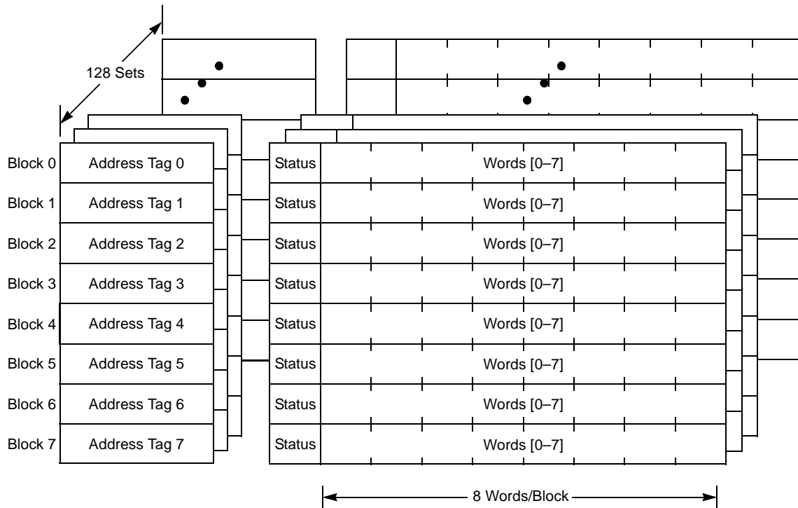
Figure 3. L1 Cache Organization
