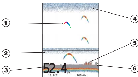
Fig. 6.6.2 - The Fish Finder Echogram
